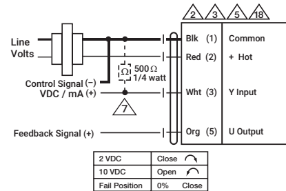
Proportional, CQKB24-SR-RR
