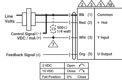
Proportional, CQKB24-SR-LR
