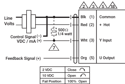
Proportional, CQKB24-SR-RL
